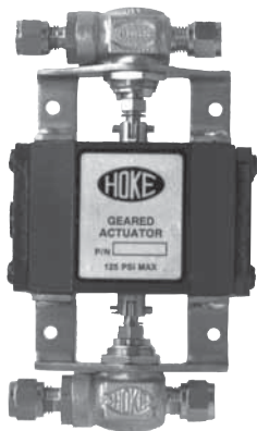
The 0700 Series single actuator offers the capability of operating up to two 2-way ball valves simultaneously.
